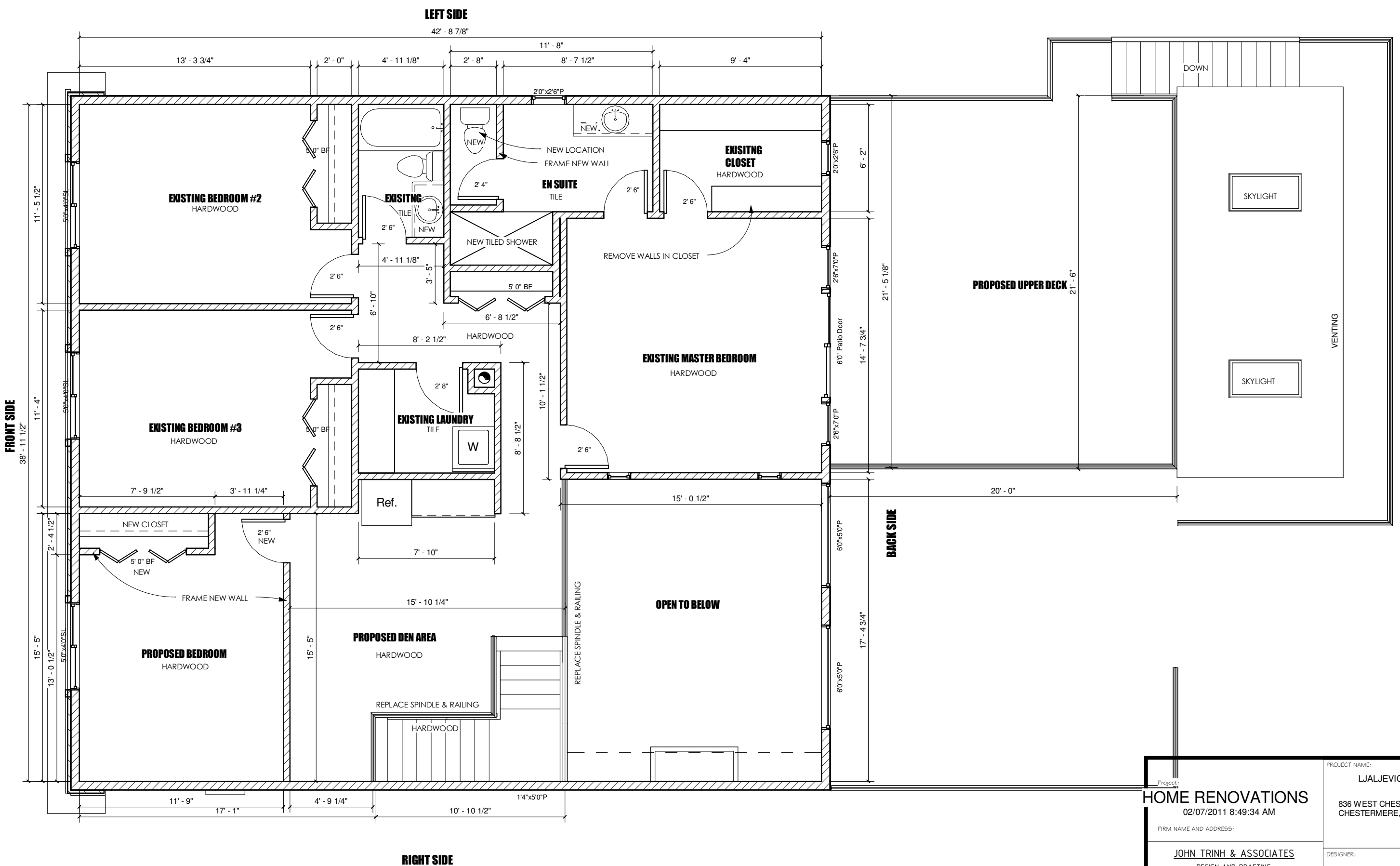
UPPER FLOOR PLAN SCALE: 3/16" = 1'-0"
