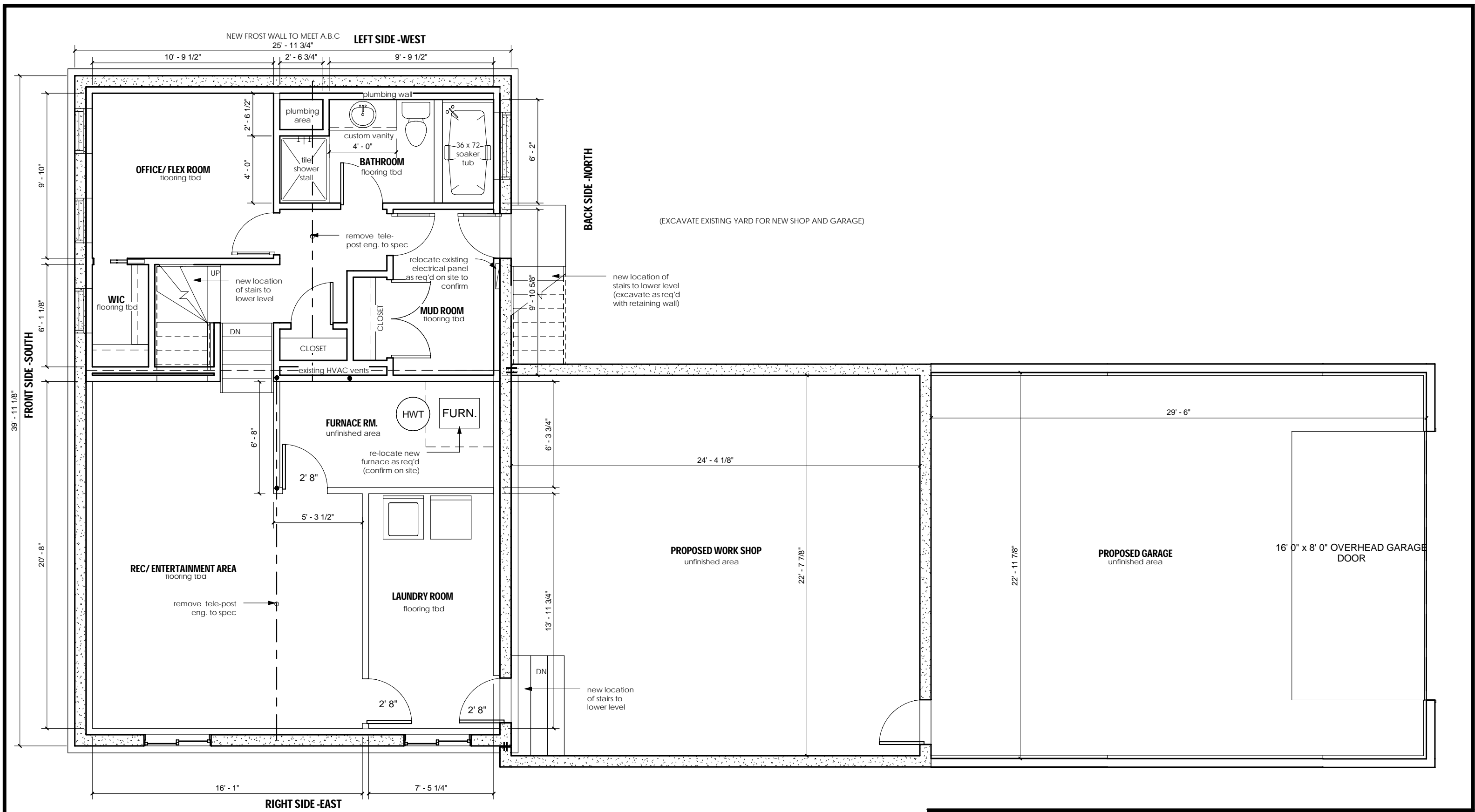
PROPOSED BASEMENT FLOOR PLAN SCALE: 3/16" = 1'-0"
