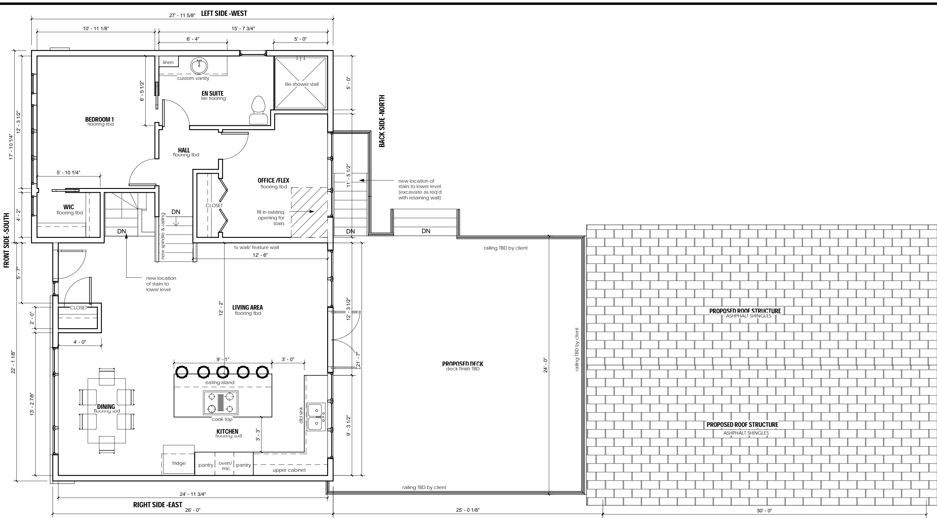
PROPOSED MAIN FLOOR PLAN SCALE: 3/16" = 1'-0"
